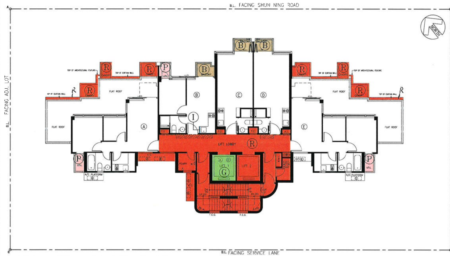
COMMON AREAS PLAN (29TH FLOOR) SCALE 1 : 200
