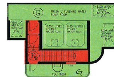
PUMP ROOM FLOOR PLAN
