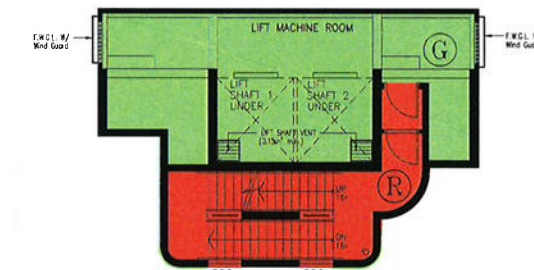
LIFT MACHINE ROOM FLOOR PLAN
