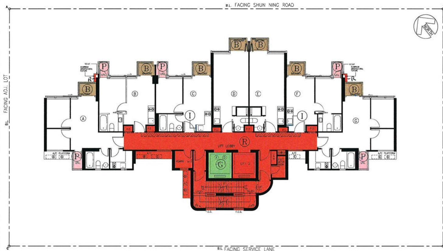
COMMON AREAS PLAN (7TH - 17TH FLOOR) SCALE 1 : 200
