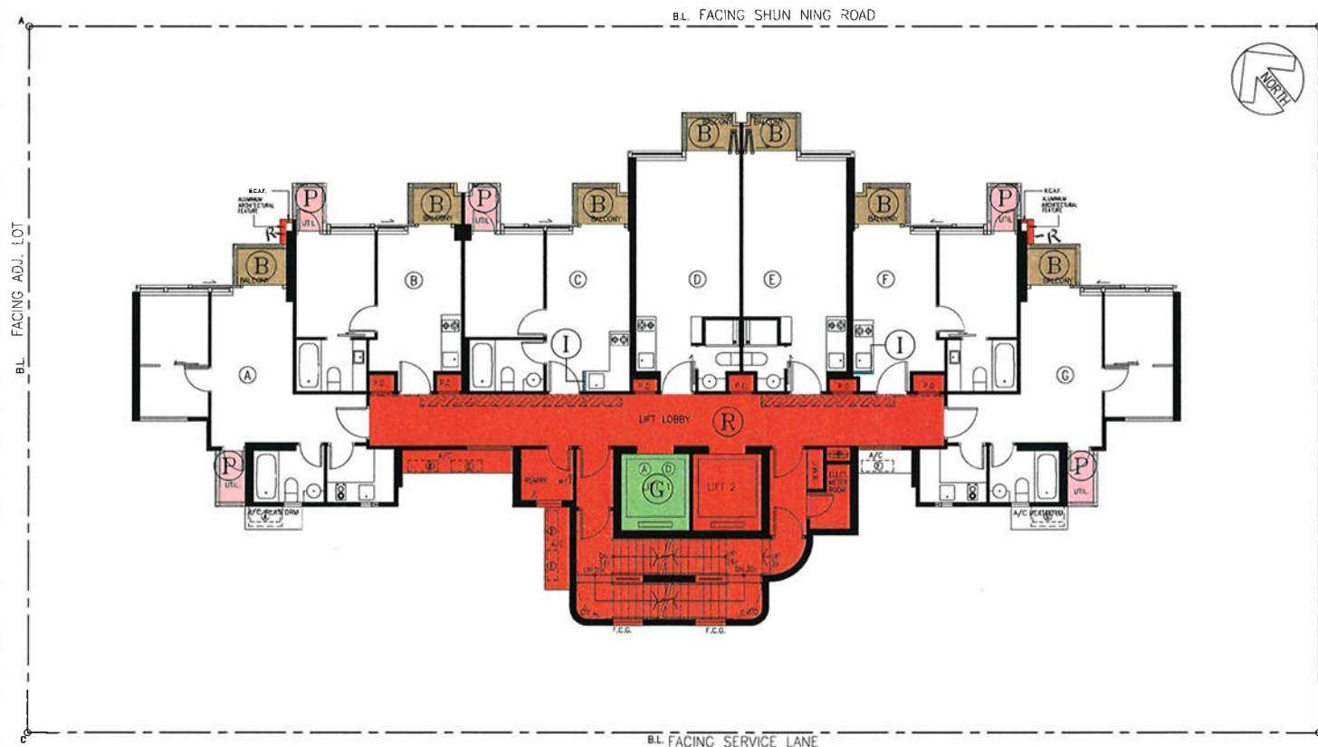
COMMON AREAS PLAN (28TH FLOOR) SCALE 1 : 200
