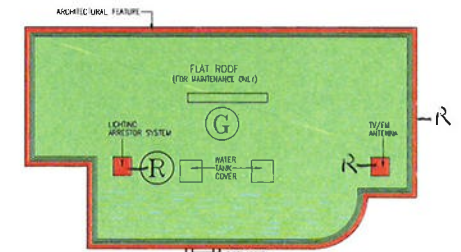
UPPER ROOF PLAN
