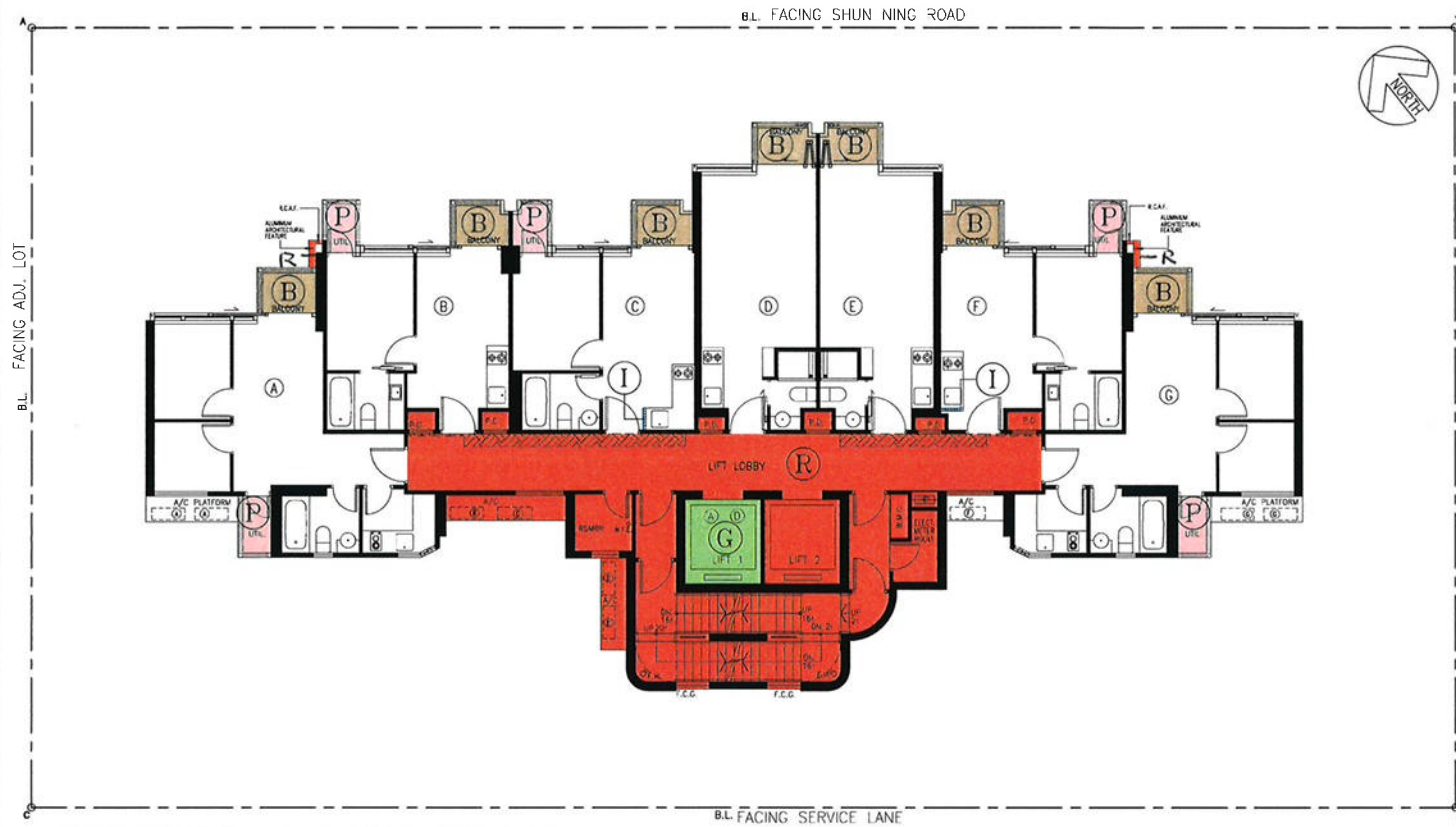
COMMON AREAS PLAN (6TH FLOOR) SCALE 1 : 200
